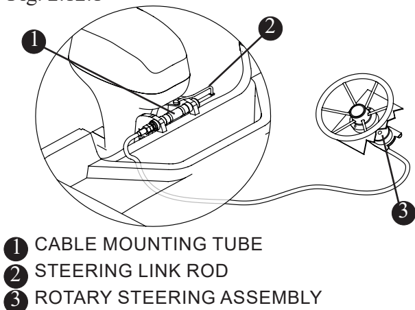
No-Feedback Steering (Typical) Fig. 2.12.1
